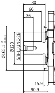
“E3” type spline shaft
