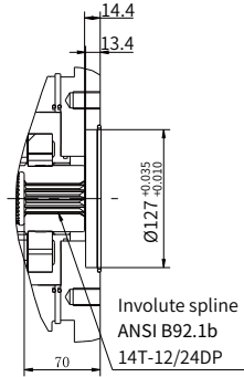
"C6" type through drive
